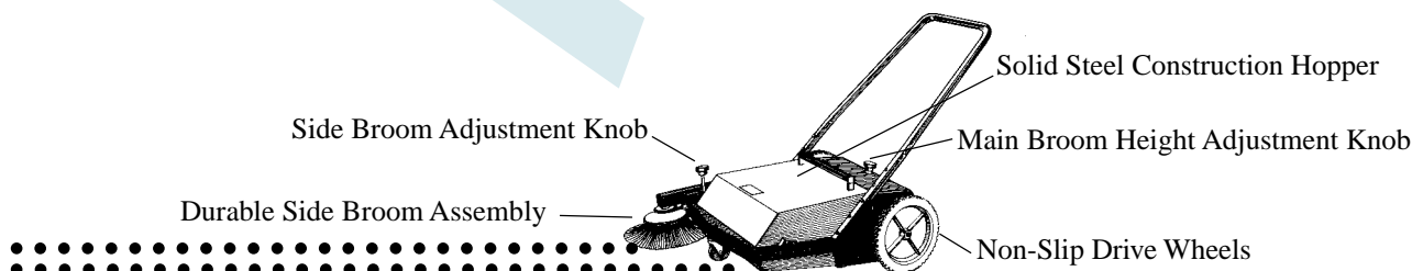
Steel hopper is easily removed to dump waste.
